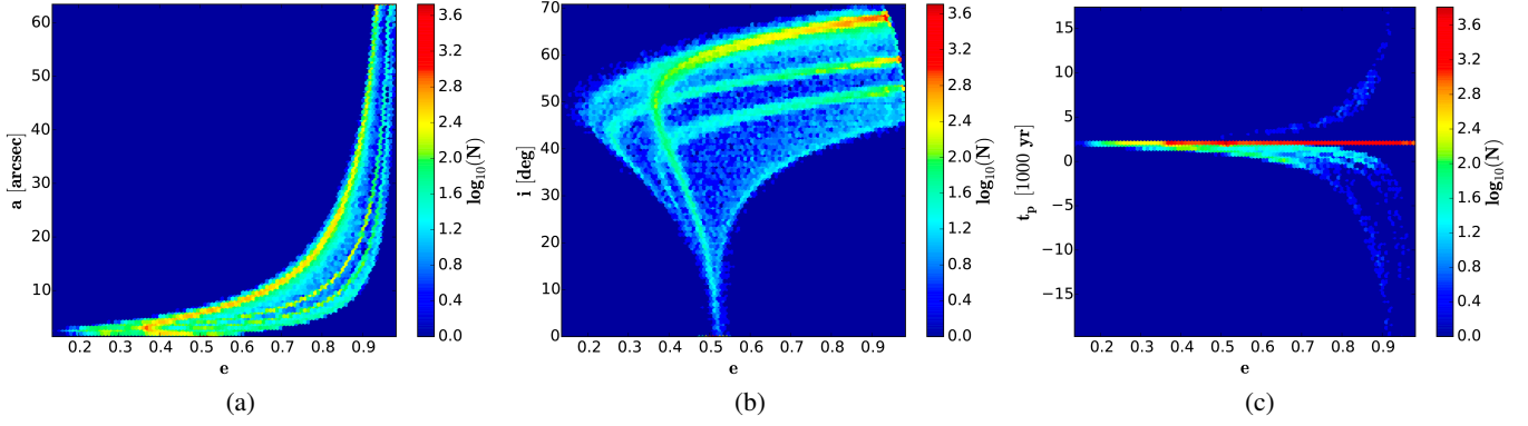
Fig. 8: Semi-major axis, inclination and time of periastron passage as function of eccentricity for all solutions with \chi_{red}^2 \leq 2 out of 5 000 000 runs of our LSMC fit. Logarithmic density of solutions is indicated by color.
