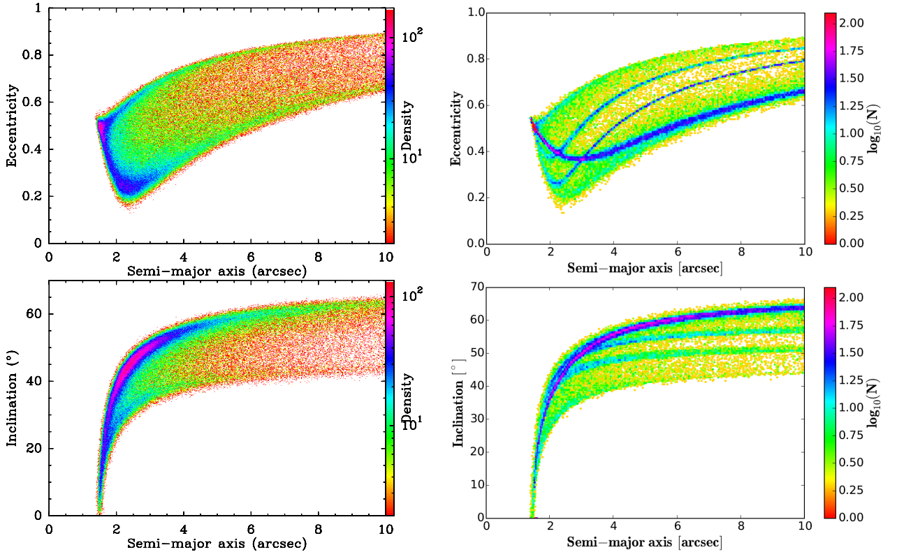
Fig. 13: Left : Additional plots to Fig. 12 restricted to bound orbits only recovered by our MCMC fit, showing bidimensional density maps involving the semi-major axis a versus the eccentricity e and the inclination i . The color scale appearing on the right side of the plots also applies to all similar plots of Fig. 12. Right : The same bidimensional density maps as shown in Fig. 13 showing orbit solutions recovered by our LSMC fit with semi-major axes smaller than 10'' .
