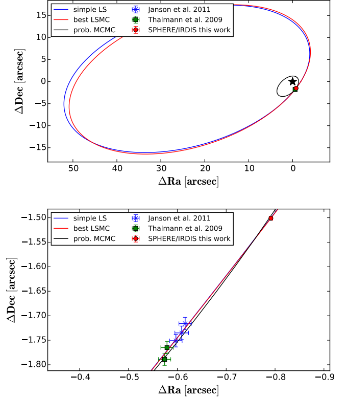
Fig. 9: Best fitting orbits recovered with simple least squares fitting as well as LSMC fitting. In addition, we show a probable orbit with orbital elements close to the peak values recovered by our MCMC fit (see Sect. 6.2). Solid lines represent the apparent orbits. The corresponding orbital elements are listed in Table 9. We show the data points taken with Subaru/HiCIAO (green squares) as given in Thalmann et al. (2009), as well as the data points taken with Subaru/HiCIAO, Gemini/NICI and Keck/NIRC2 (blue crosses) given in Janson et al. (2011) together with our SPHERE/IRDIS measurement (red circle).
