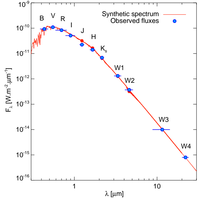
Fig. 3: GAIA-COND synthetic spectrum adjusted onto the spectral energy distribution of GJ 758 A built from a compilation of optical, near-infrared, and mid-infrared photometry. The 2MASS J , H , K_s and WISE W1–W2 photometry data were excluded from the fit because the star was saturating in the 2MASS images.
