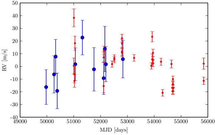
Fig. 11: Radial velocity measurements of GJ 758 A, retrieved from the ELODIE (large blue dots) and Lick Planet Search (small red dots) archives. The measurements cover a total of 16 years which is nearly the full period of the inner companion speculated from the astrometric signal.
