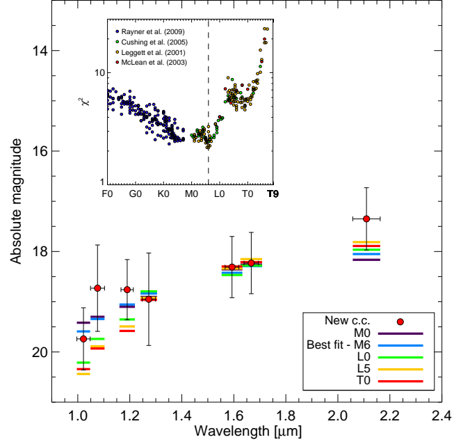
Fig. 7: Comparison of the absolute magnitudes of the newly identified candidate (red circles) with photometry of different stellar and sub-stellar objects from various libraries (Leggett et al. 2001; McLean et al. 2003; Cushing et al. 2005; Rayner et al. 2009). The inset plot at the top shows the \chi^2 values as a function of spectral type, which shows a minimum for M6.
