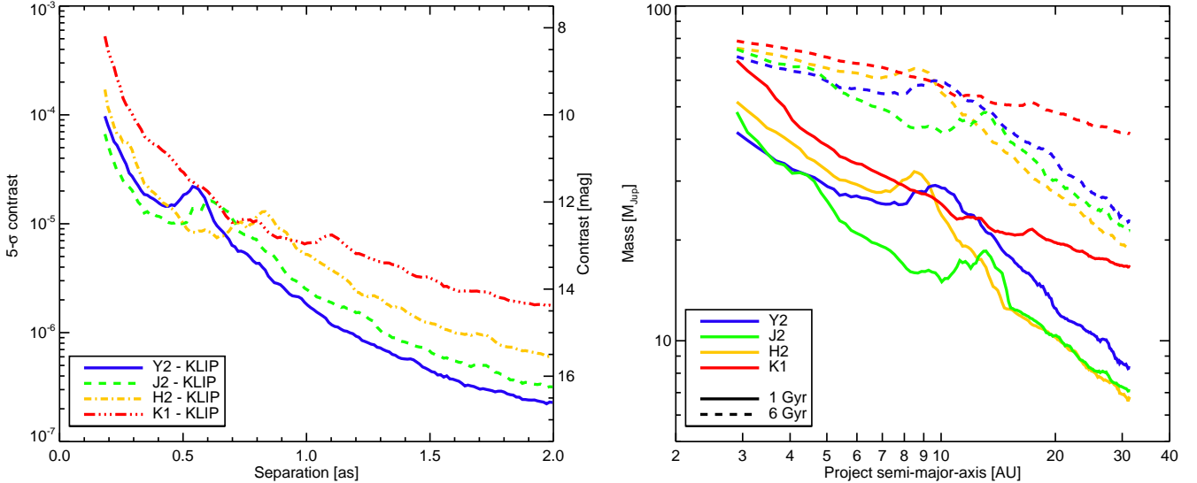
Fig. 14: Left : 5\text{-}\sigma detection limits measured in the Y2, J2, H2 and K1 filters using a KLIP analysis, with a number of subtracted modes that varies to maximize the algorithm throughput. Right : Conversion of these detection limits into physical units using the known distance of the GJ 758 system (15.76 pc) and the AMES-COND evolutionary tracks (Baraffe et al. 2003) calculated in the IRDIS filters. Two sets of curves assuming the two extremes of the system age range (1 and 6 Gyr, see Sect. 4) are displayed. The limits for the nominal age of 3 Gyr lie in-between, slightly closer to the the 6 Gyr limit than the 1 Gyr limit.
