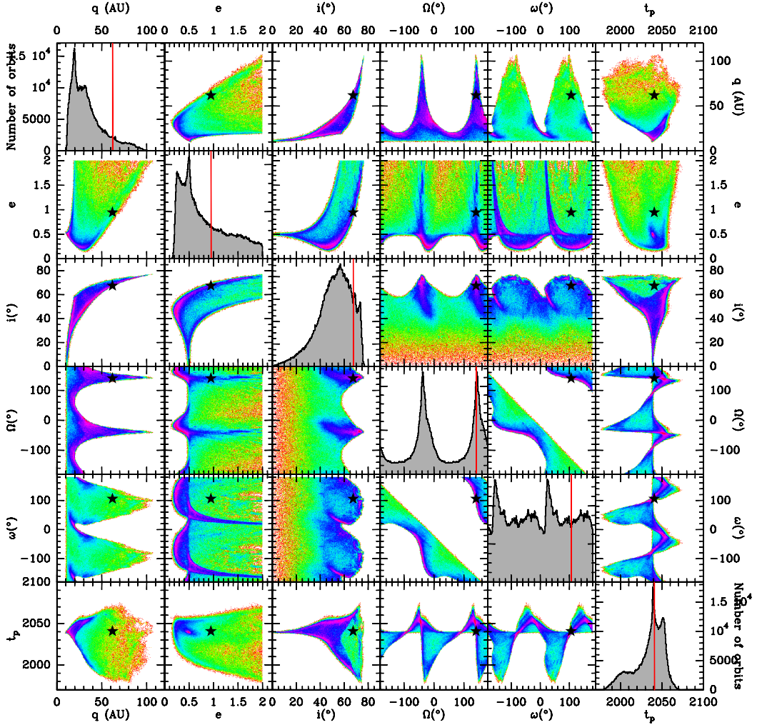
Fig. 12: Resulting MCMC posterior distribution of the six orbital elements ( q , e , i , \Omega , \omega , t_p ) of GJ 758 B’s orbit using the universal variable code. The diagonal diagrams show mono-dimensional probability distributions of the individual elements. The off-diagonal plots show bidimensional probability maps for the various couples of parameters. This illustrates the correlation between orbital elements. The logarithmic color scale in these plots is linked to the relative local density of orbital solutions. It is indicated on the side of Fig. 13. In the diagonal histograms, the red bar indicates the location of the best \chi^2 solution obtained via standard least-square fitting. The location of this solution is marked with black stars in the off-diagonal plots. This solution is also plotted in Fig 9.
