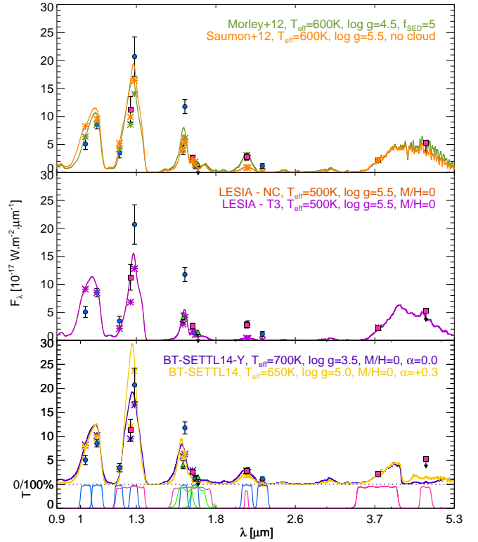
Fig. 5: Comparison of the 1–5 \mu\text{m} spectral-energy distribution of GJ 758 B to the best fitting synthetic spectra from the BT-SETTL14, Morley+12, Saumon+12, and LESIA model grids.
