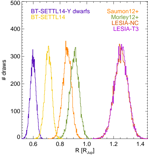
Fig. 6: Histogram of radii (dilution factors C_k , directly related to radius because the distance is known) derived from the comparison of the most frequent best-fitting solution for each Monte-Carlo simulation of the SED of GJ 758 B.
