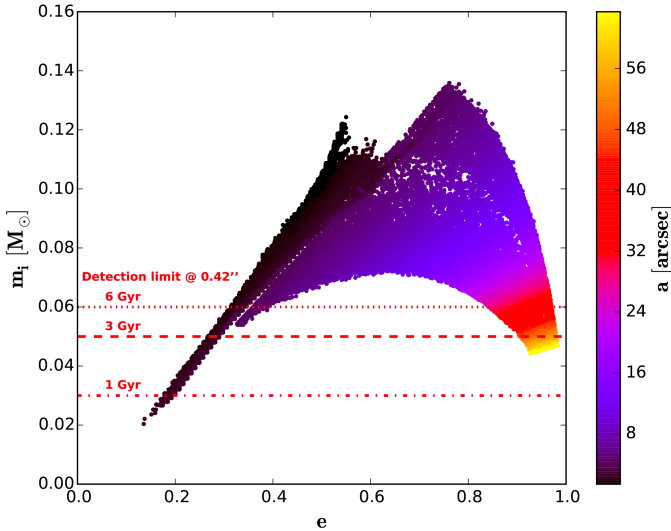
Fig. 10: Minimum mass of an unseen inner companion that would cause a false positive eccentricity signal in the relative astrometry of GJ 758 A and B by astrometric displacement of GJ 758 A due to their common orbit around the center of mass of the system. The minimum mass is a function of the eccentricity and semi-major axis of the A/B system as well as the maximum epoch difference of all astrometric measurements. Shown are such minimum masses for all orbits with \chi_{red}^2 \leq 2 which were recovered for the A/B system. Using our deep SPHERE/IRDIS observations as well as the AMES-COND models Baraffe et al. (2003) we also show the detectable minimum mass at the angular separation at which such a putative inner companion would need to reside. We can exclude the presence of an object that would introduce a false positive eccentricity in all cases.
