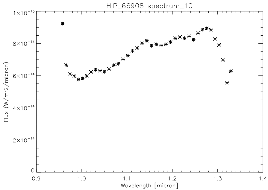
Figure 8 – Spectrum extracted for HIP 66908
