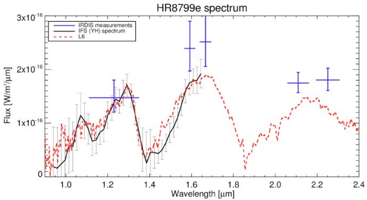
Figure 11 – Extracted spectrum for HR8799e
