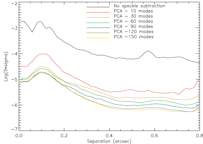
Figure 2: 5-sigma contrast curves from the COM2 Y-J image of HR7581 obtained using PCA-based differential imaging. The curves were corrected for cancellation effects using fake planets.
