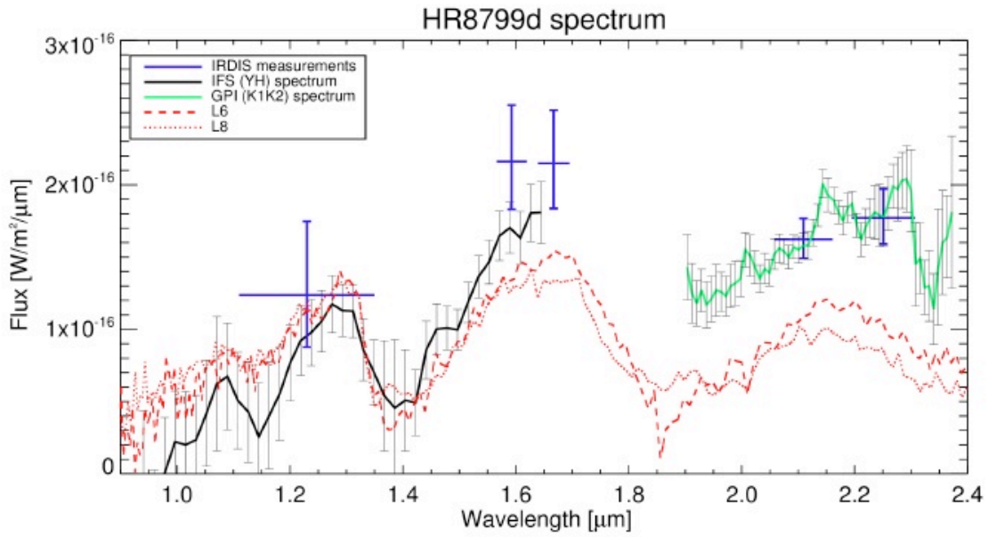
Figure 10 – Extracted spectrum for HR8799d
