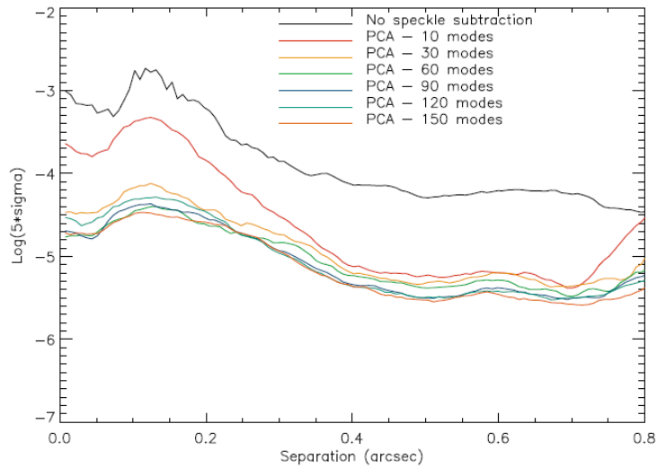
Figure 5: Same as Figure 2. The target star is \epsilon Sgr.
