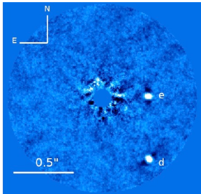
Figure 9 – Final image of the inner part of the HR 8799 system where the two innermost planets are clearly visible
