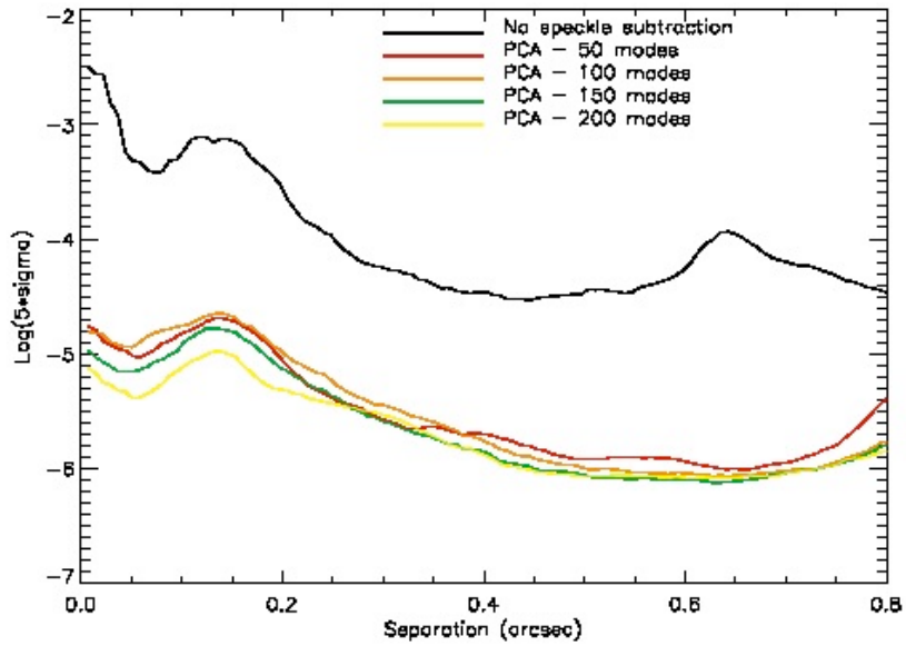
Figure 6 - Contrast plot for Sirius obtained with different number of principal components for the PCA
