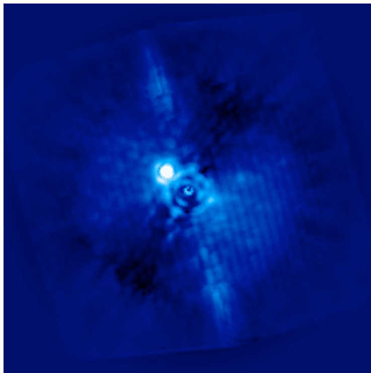
Figure 7 – Final image for HIP 66908
