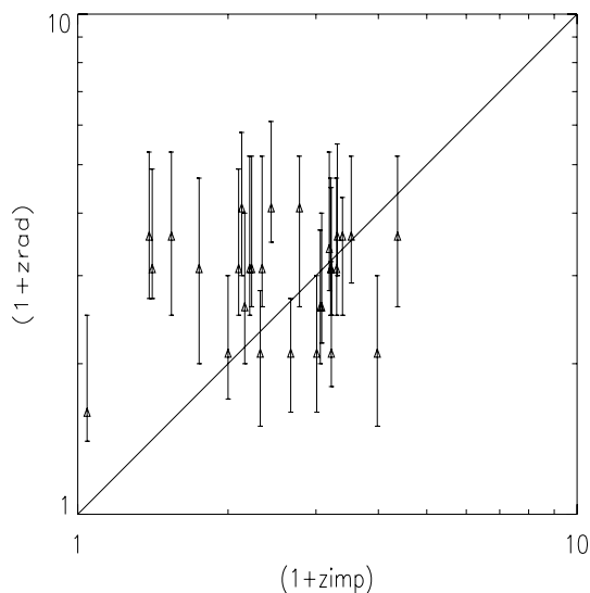
Figure 2. Comparison of current redshift estimations and those using radio-far-IR Fluxes. Comparison between the photometric redshifts obtained here ( z_{\text{imp}} ) with those obtained by Artxega et al. (2007) using a radio-far-IR based method ( z_{\text{rad}} ). The error bars shown are 1\sigma uncertainties. We use their z_{\text{phot}}^A parameter for this plot.
