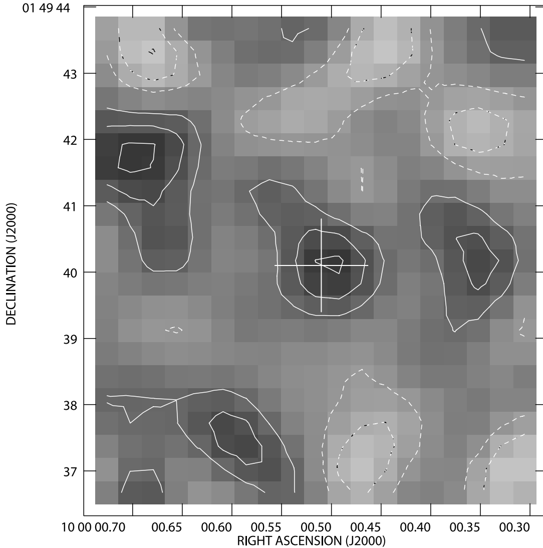
FIG. 2.—VLA 1.4 GHz image of the field centered on the z = 5.7 LAE J10000.51+014940.1 in Ajiki et al. (2006). The cross marks the position of the LAE. The contour levels are -27, -18, -9, 9, 18, and 27 \mu\text{Jy beam}^{-1} , and the beam has \text{FWHM} = 1.5'' .
