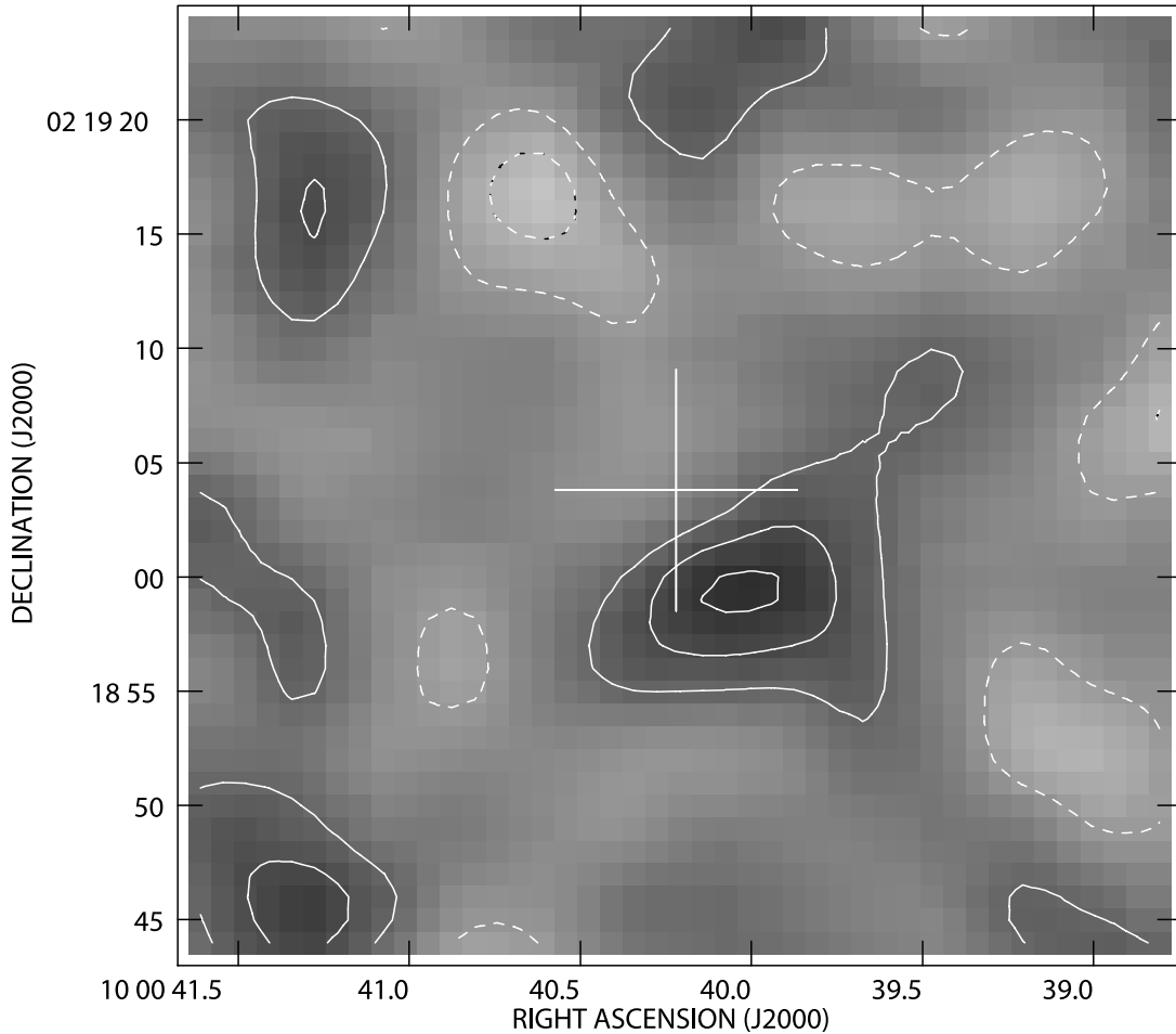
FIG. 3.—MAMBO 250 GHz image of the field centered on the z = 5.7 LAE J100040.22+021903.8 in Ajiki et al. (2006). The cross marks the position of the LAE, and the size of the cross corresponds to the FWHM of the MAMBO beam. The contour levels are -3, -2, -1, 1, 2, and 3 \text{ mJy beam}^{-1} , and the beam has \text{FWHM} = 10.6'' .
