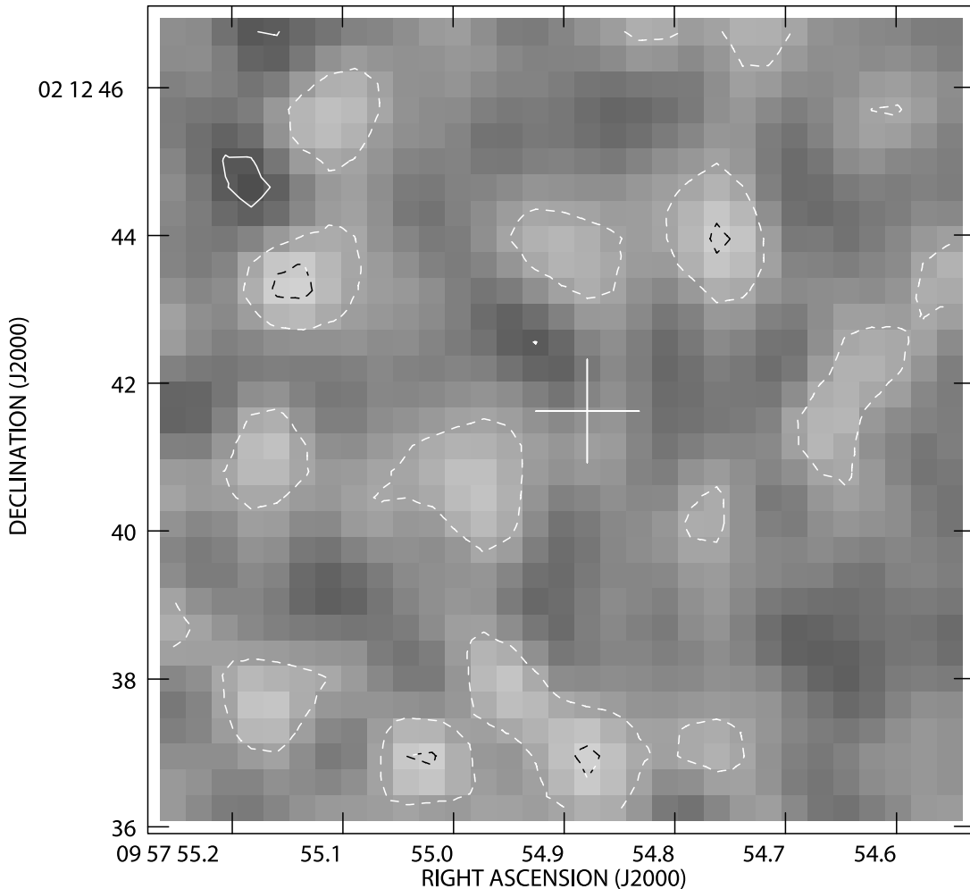
FIG. 1.—Stacked 1.4 GHz image of the LAEs in the COSMOS field (99 sources). The rms noise level is 1.25 \mu\text{Jy beam}^{-1} . The cross marks the stacking position, centered on the LAE positions (the absolute coordinates are arbitrary). The contour levels are -6, -4, -2, 2, 4, and 6 \mu\text{Jy beam}^{-1} , and the beam has \text{FWHM} = 1.5'' .
