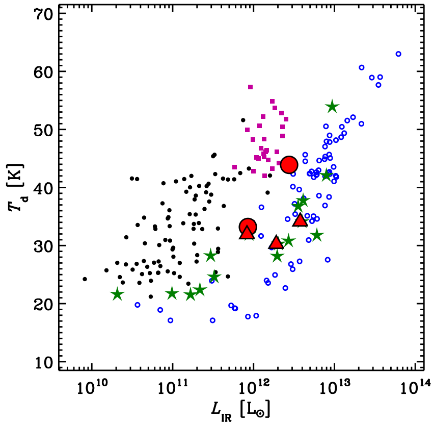
Fig. 4.— The IR luminosity-dust temperature distribution for various IR-luminous galaxy samples. For the 350\ \mu\text{m} -selected galaxies, the red circles show SSG 1 and SSG 2, and triangles show LH 350.1, 350.2, and 350.3. Green stars represent the 850 and 1100\ \mu\text{m} -selected SMGs for which there is 350\ \mu\text{m} follow-up photometry. This is compared with 850\ \mu\text{m} -selected SMGs from Chapman et al. (2005) (open blue circles) and IRAS galaxies from Dunne et al. (2000) (filled black squares) and Clements et al. (2009) (purple squares).
