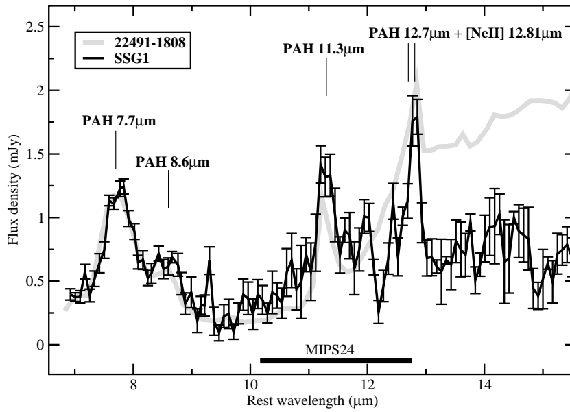
Fig. 1.— The mid-IR spectrum of SSG 1 as observed by Spitzer IRS, indicated by black line. One-sigma error bars are shown. Wavelengths are in the rest frame based on the derived redshift z = 1.05 . The spectrum of IRAS 22491–1808, used as a template to derive the redshift, is shown in grey. Prominent dust grain emission features are also indicated. The MIPS 24 \mu\text{m} passband is shown by the heavy black line below the spectrum.
