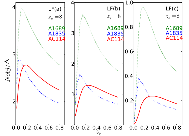
Fig. 6. Expected number of objects as a function of the cluster redshift for a fixed redshift of sources ( z_s = 8 ) and with the same depth and field size as in previous section. Three cluster models are displayed: A1689 (green dotted line), A1835 (blue dot-dashed line) and AC114 (red solid line). Panels from left to right display respectively LF (a), (b) and (c).
