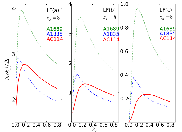
Fig. 6. Expected number of objects as a function of the cluster redshift for a fixed redshift of sources ( z_s = 8 ) and with the same depth and field size as in previous section. Three cluster models are displayed: A1689 (green dotted line), A1835 (blue dot-dashed line) and AC114 (red solid line). Panels from left to right display respectively LF (a), (b) and (c).
