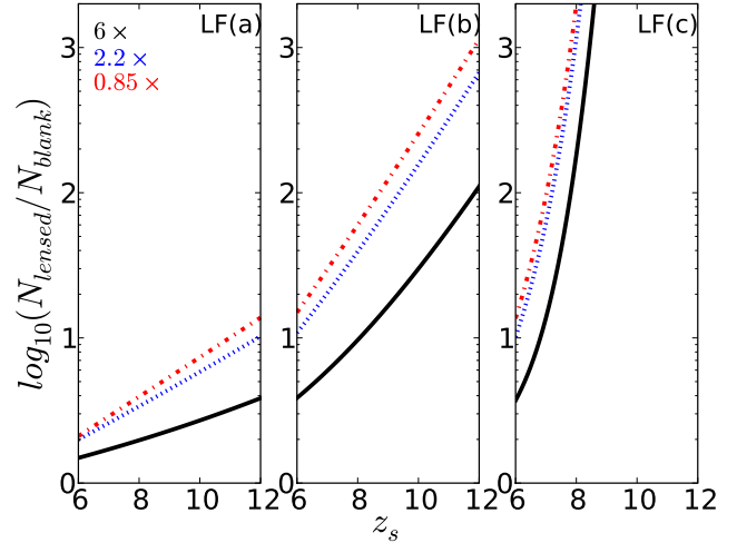
Fig. 3. Relative gain in number counts between lensing and blank fields as a function of the source redshift, with \Delta z = 1 , for different fields of view: 6' \times 6' in black, 2.2' \times 2.2' in blue dotted line and 0.85' \times 0.85' in red dot-dashed line (from bottom to top). The three panels from left to right represent the 3 values of the LF, (a), (b) and (c) respectively.
