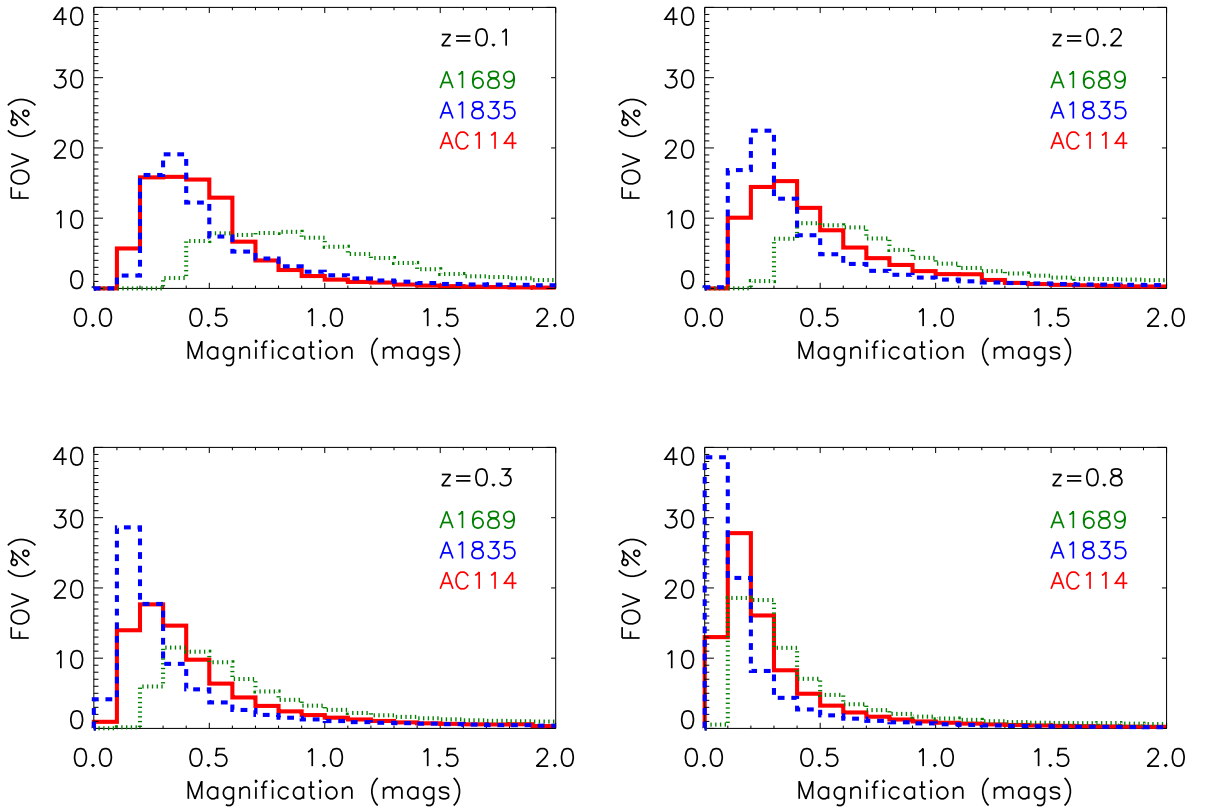
Fig. 7. Histogram representing the percentage of the surface ( 6' \times 6' FOV) as a function of the magnification for different redshifts of cluster ( z_c=0.1, 0.2, 0.3, 0.8 ), using the same color codes for the three clusters as in Fig. 6 (A1689: green dotted line, A1835: blue dot-dashed line and AC114: red solid line)
