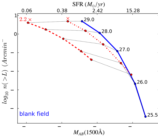
Fig. 12. Cumulative surface density of sources as a function of their intrinsic UV luminosity and SFR, in blank fields (blue solid line) and in the lensing fields with FOV 6' \times 6' (red dotted line) and 2.2' \times 2.2' (JWST-like, red dashed line), for different photometric depths ranging from shallow ( AB \sim 25.5 ) to deep ( AB \sim 29.0 ) surveys and a strongly evolving LF(c). The mean magnification over the whole the field is used to derive the lensing points, the true distribution is displayed in Fig. 11. The source redshift is arbitrarily fixed at z=8 , with \Delta z = 1 . The conversion from absolute magnitude to SFR is provided in Sect. 2.1.3 using the calibrations from ?.
