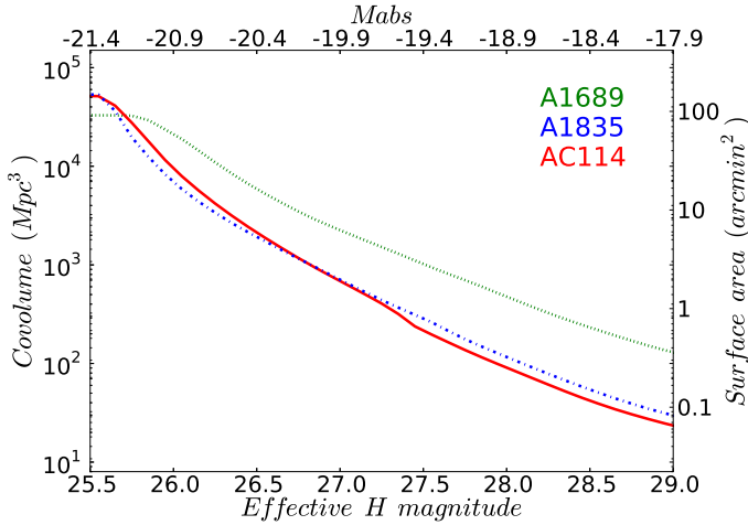
Fig. 8. The effective (lensing corrected) covolume sampled at z=6.5-7.5 by each cluster is given as a function of effective H_{AB} magnitude limit, for a magnitude-limited survey of 6' \times 6' FOV with H_{AB} \leq 25.5 . The three clusters are displayed with the same colors and line codes as in Fig. 6.
