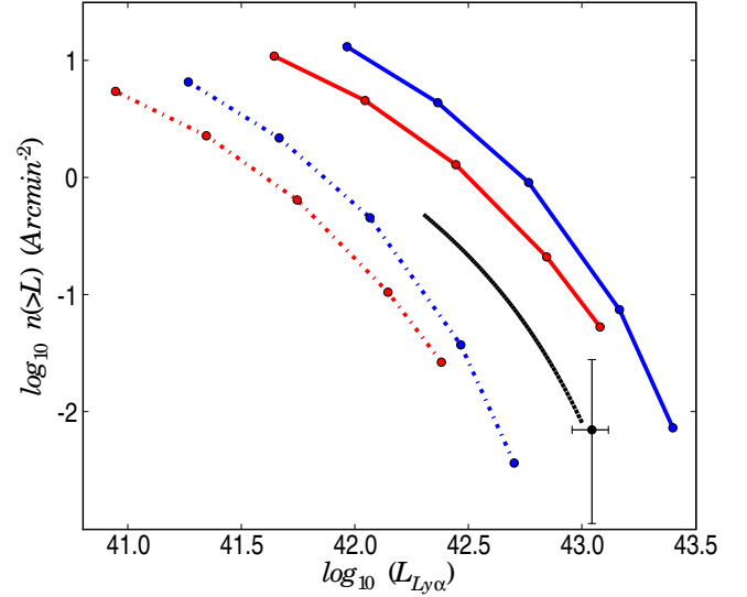
Fig. 13. Cumulative surface density of observed sources as a function of their Lyman alpha luminosity ( 6' \times 6' FOV, \Delta z = 1 , redshift of sources fixed at 6.6 for the LF(c)). The density is calculated in blank (blue solid line) and in lensing fields (red solid line) for different limiting magnitudes (from right to left: 25.5, 26.0, 27.0, 28.0 and 29.0). Dashed lines display number counts corrected by transmission value \epsilon \sim 10\% (dashed red line in lensing fields and dashed blue line in blank field). For comparison, raw number counts extracted from the spectroscopic sample of LAEs by ? are also given (black solid line). The number density derived from ? at z = 6.96 is also indicated, together with corresponding error bars (see text for details). As in Fig. 12, the magnification used to derive the lensing points is averaged over the entire field.
