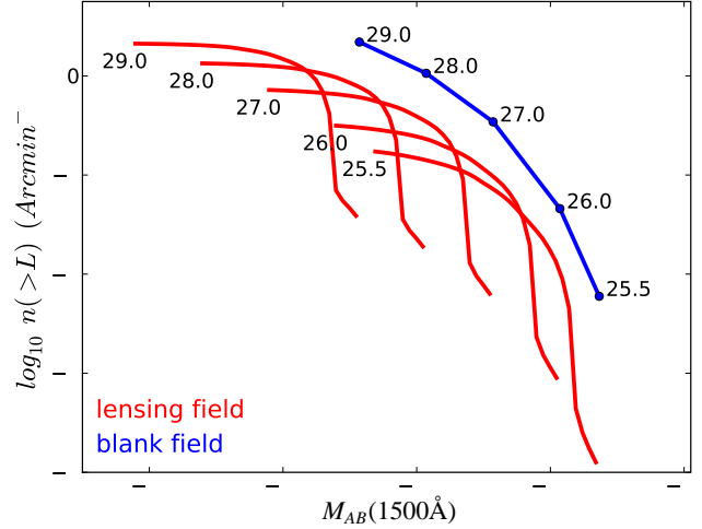
Fig. 11. Cumulative surface density of sources as a function of their intrinsic UV luminosity, in blank fields (blue solid line) and in the lensing fields with FOV \sim 5 arcmin ^2 (JWST-like, red solid line), for different photometric depths ranging from shallow ( AB \sim 25.5 ) to deep ( AB \sim 29.0 ) surveys and a strongly evolving LF(c). The source redshift is arbitrarily fixed at z=8 , with \Delta z = 1
