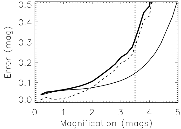
Fig. 2. Typical error in the magnification factor \mu , as a function of the magnification for Abell 1835. The solid curve gives the statistical error derived from the MCMC model, while the dashed curve gives the systematic error between two choices of parametrization (see text for details). The thick solid curve is the quadratic sum of both errors, used later in the calculation. The vertical line represents the conservative upper limit of \mu=25 .
