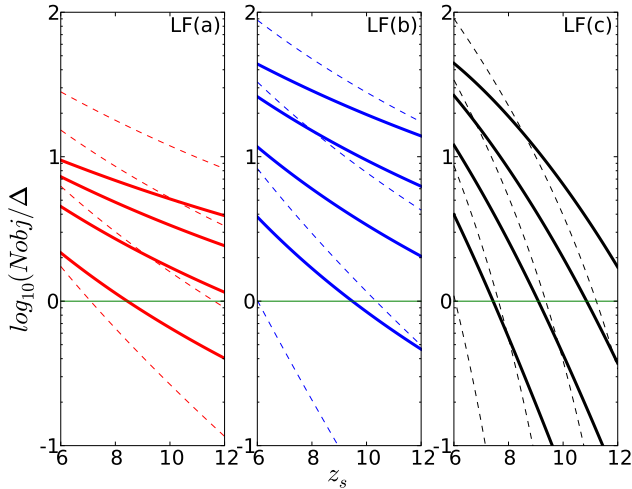
Fig. 10. The same as Fig. 9 but for a 2.2' \times 2.2' FOV. Some differences appear in comparison with the Fig. 9. For example, the total numbers of high- z galaxies expected behind lensing clusters (solid lines) and the field (dashed lines) are much larger at low limiting magnitude ( m_{AB} = 26.0 ) but this phenomenon is reversed for deeper surveys ( m_{AB} = 28.0 - 29.0 ) (see text for details).
