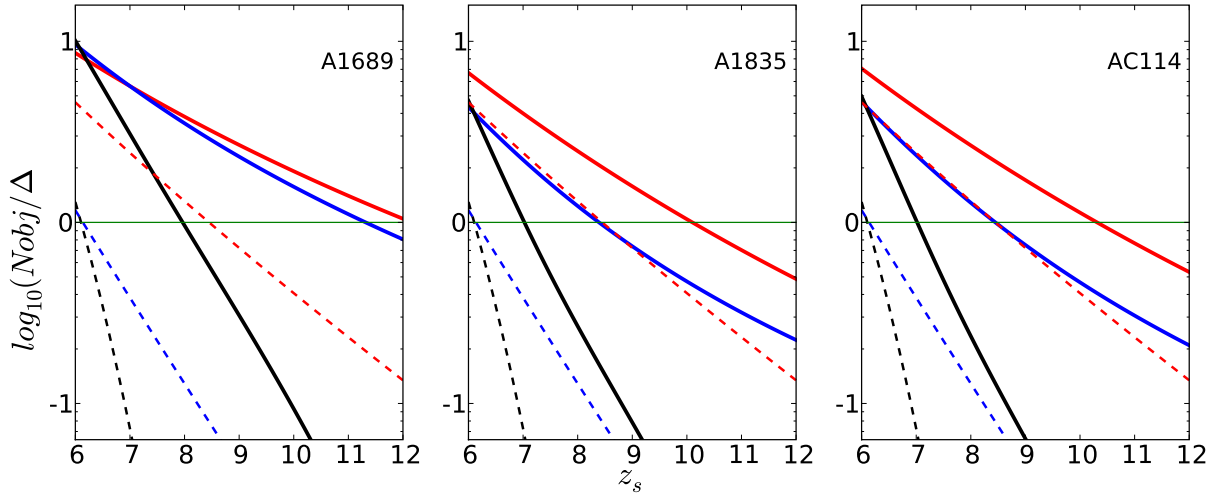
Fig. 4. Comparison between the expected number counts of galaxies in a typical 6' \times 6' FOV, up to H_{AB} \leq 25.5 , per redshift bin \Delta z = 1 , in a blank field (dashed lines) and in the field of lensing cluster (solid lines) (left to right respectively A1689, A1835 and AC114). Expected counts are obtained by the integration of 3 different luminosity functions (a), (b) and (c) from top to bottom. The limit of one source detected in the field of view is indicated by an horizontal line to guide the eye.
