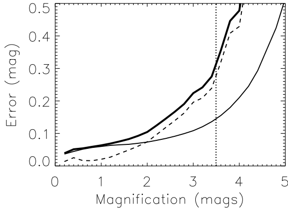
Fig. 2. Typical error in the magnification factor \mu , as a function of the magnification for Abell 1835. The solid curve gives the statistical error derived from the MCMC model, while the dashed curve gives the systematic error between two choices of parametrization (see text for details). The thick solid curve is the quadratic sum of both errors, used later in the calculation. The vertical line represents the conservative upper limit of \mu=25 .
