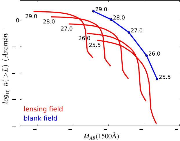
Fig. 11. Cumulative surface density of sources as a function of their intrinsic UV luminosity, in blank fields (blue solid line) and in the lensing fields with FOV \sim 5 arcmin ^2 (JWST-like, red solid line), for different photometric depths ranging from shallow ( AB \sim 25.5 ) to deep ( AB \sim 29.0 ) surveys and a strongly evolving LF(c). The source redshift is arbitrarily fixed at z=8 , with \Delta z = 1
