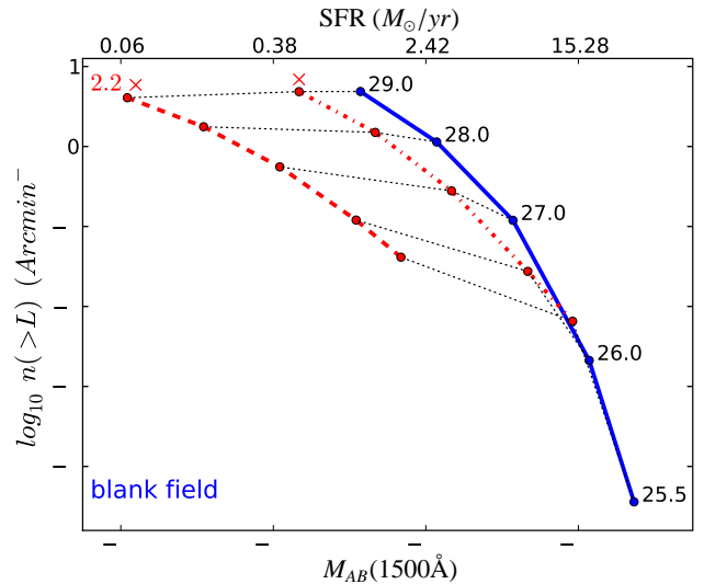
Fig. 12. Cumulative surface density of sources as a function of their intrinsic UV luminosity and SFR, in blank fields (blue solid line) and in the lensing fields with FOV 6' \times 6' (red dotted line) and 2.2' \times 2.2' (JWST-like, red dashed line), for different photometric depths ranging from shallow ( AB \sim 25.5 ) to deep ( AB \sim 29.0 ) surveys and a strongly evolving LF(c). The mean magnification over the whole the field is used to derive the lensing points, the true distribution is displayed in Fig. 11. The source redshift is arbitrarily fixed at z=8 , with \Delta z = 1 . The conversion from absolute magnitude to SFR is provided in Sect. 2.1.3 using the calibrations from Kennicutt (1998).
