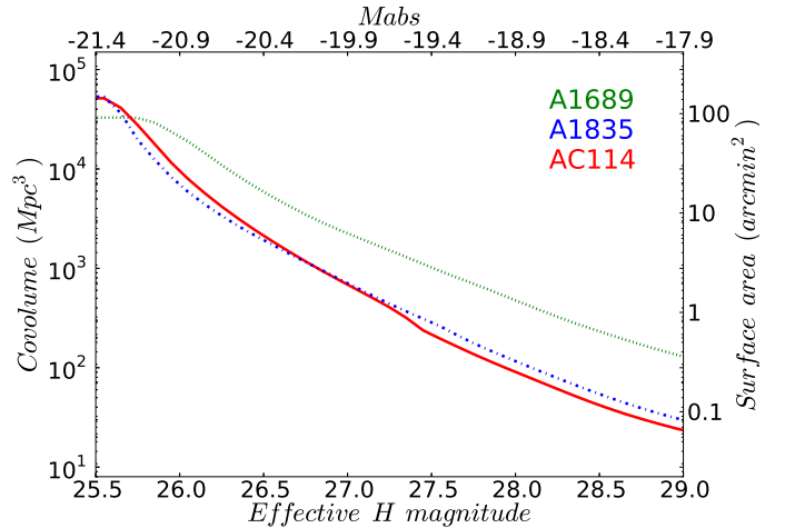
Fig. 8. The effective (lensing corrected) covolume sampled at z=6.5-7.5 by each cluster is given as a function of effective H_{AB} magnitude limit, for a magnitude-limited survey of 6' \times 6' FOV with H_{AB} \leq 25.5 . The three clusters are displayed with the same colors and line codes as in Fig. 6.
