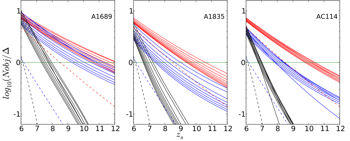
Fig. 5. The same as Fig. 4 but using different assumptions for the redshift of the clusters, with z_c \in [0.1, 0.8] and a 0.1 step (for more details see Sect. 3.3)
