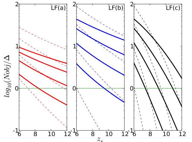
Fig. 10. The same as Fig. 9 but for a 2.2' \times 2.2' FOV. Some differences appear in comparison with the Fig. 9. For example, the total numbers of high- z galaxies expected behind lensing clusters (solid lines) and the field (dashed lines) are much larger at low limiting magnitude ( m_{AB} = 26.0 ) but this phenomenon is reversed for deeper surveys ( m_{AB} = 28.0 - 29.0 ) (see text for details).
