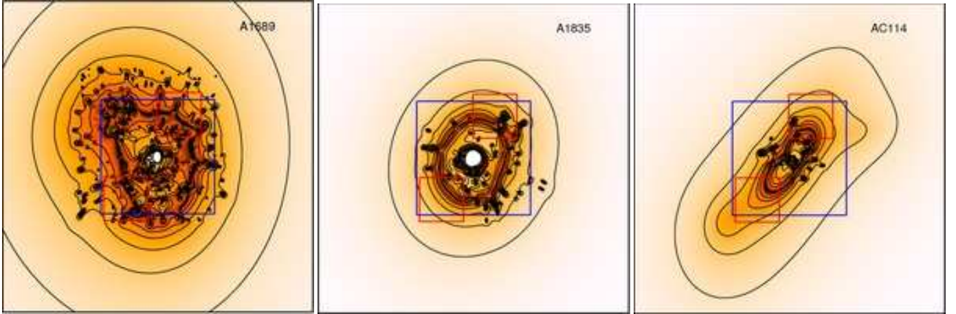
Fig. 1. Magnification maps for the three clusters at z_s = 8 used in this study (from left to right A1689, A1835 and AC114 respectively). The global size of the image corresponds to the 6' \times 6' FOV whereas the blue and red squares correspond respectively to 2.2' \times 2.2' and 0.85' \times 0.85' FOV (see Sect. 2.1.3). Black contours represent different magnification regimes with increasing magnification values from 0.5 to 3 mags towards the cluster center.
