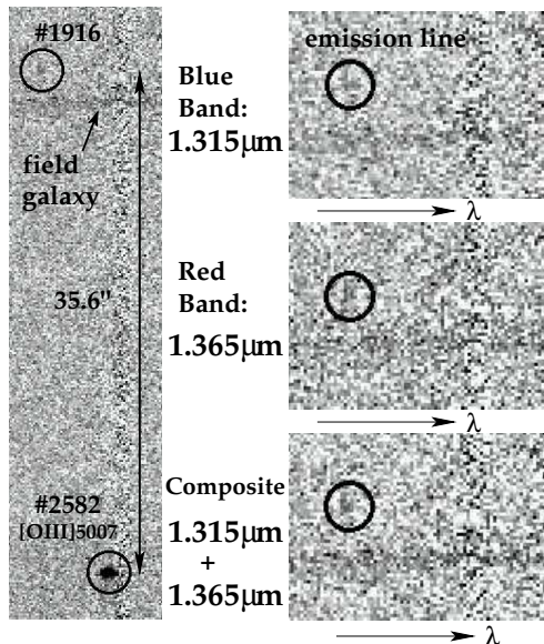
Fig. 4. 2D spectra showing the detected emission line of #1916, as well the nearby field galaxy and the [O III] \lambda 5007 line of the galaxy #2582 ( z = 1.68 ) used as a reference to stack the data sets. 2D spectra are sky subtracted and show the spectral region around the emission-line at 1.33745 \mu\text{m} , leading to z = 10.00175 \pm 0.00045 when identified as \text{Ly}\alpha(1215.67 \text{ \AA}) . The line is seen on the 2 independent overlapping bands at 1.315 and 1.365 \mu\text{m} . No smoothing was applied to these spectra. Both the object #2582 and the nearby field galaxy are identified in Fig.1.
