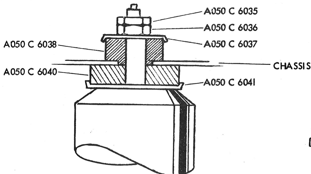
Fig. 8. DAMPER TOP MOUNTING RUBBERS
