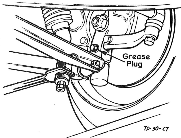
Fig. 6. VERTICAL LINK GREASE POINT.
