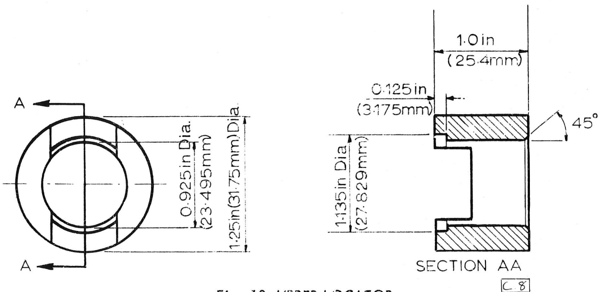
Fig. 10 UPPER LOCATOR
