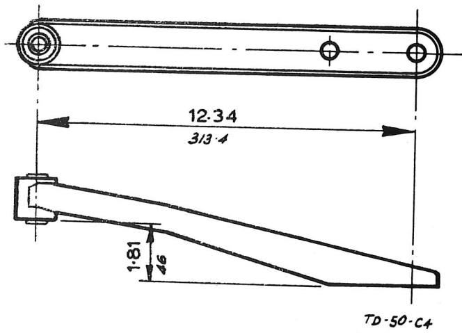
Fig. 4. LOWER WISHBONES
