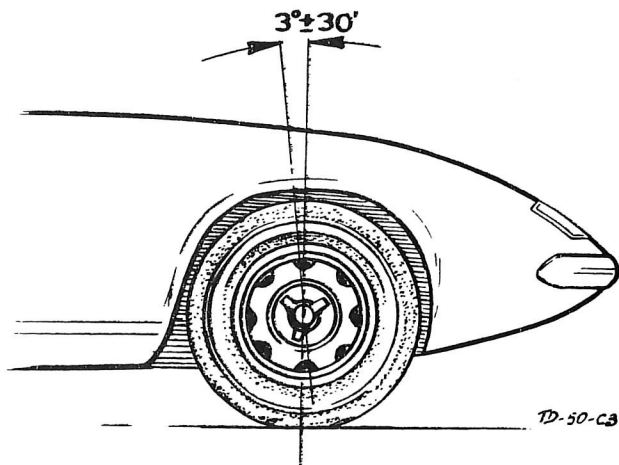
Fig. 3. CASTOR ANGLE
