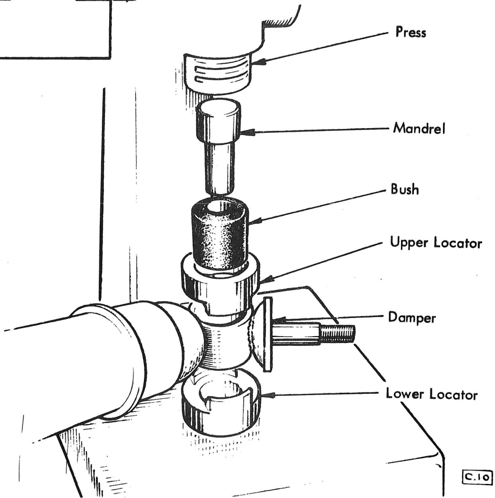
Fig. 12 REPLACING BUSH
