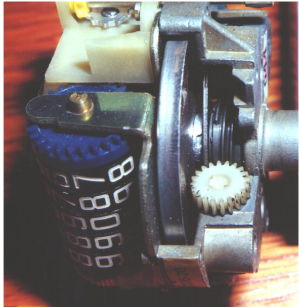
Figure 17. A view of the front of an "Old-style" speedometer. Note the separate odometer drive gears for each wheel set. Also note the all metal construction. The trip odometer wheels are set immediately next to each other in contrast to later speedometers such as the new-style one in the earlier photographs (fig. 2). The shaft on the right is the trip odometer reset. The return spring is not in the same place as the later speedometer. It is just above the pointer under the odometer wheels.
