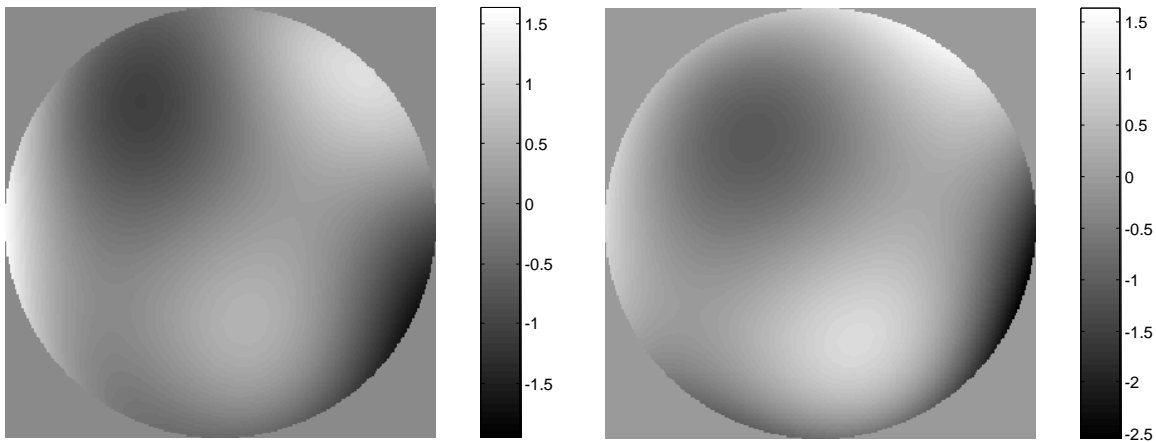
Figure 8. At left is a phase map recorded by the PSI installed as an integral part of the top box. The agreement with the phase reconstruction from the WFS at right is excellent.
